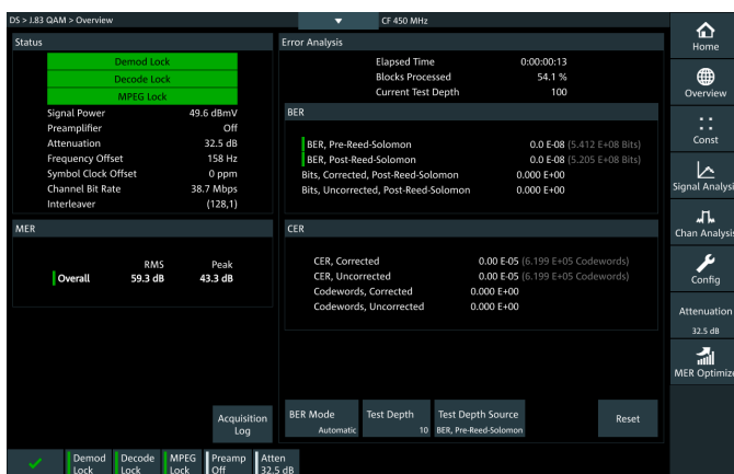
J.83 overview
