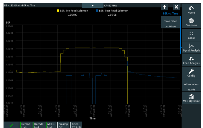
J.83 BER versus time with sporadic errors
