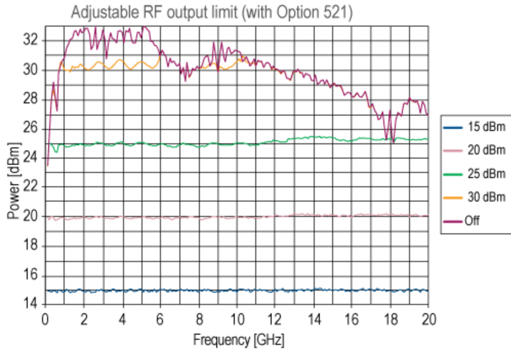
RF output limit (measured)
