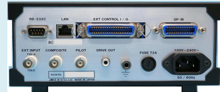
Rear panel
