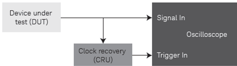
Figure 3. Clock recovery provides a compliant trigger signal for use by an oscilloscope or BERT.
