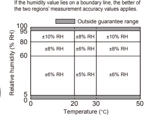
Humidity Sensor 9701 Operating temperature and humidity range: 0°C to 50°C (32°F to 122°F), 100% RH or less (non-condensing)
